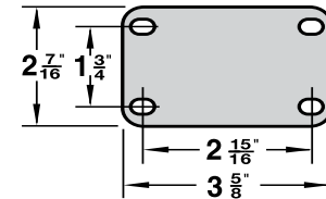
Swivel Caster
