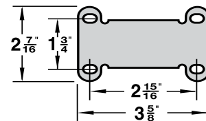
Rigid Caster
